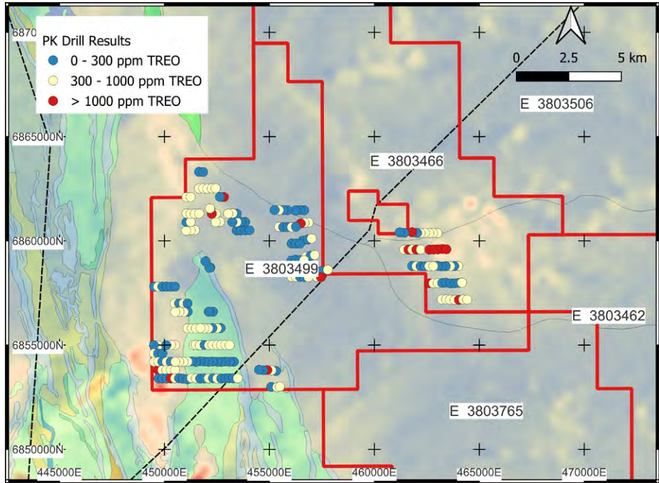
Figure 11: Point Kidman drilling results on geology/thorium image
